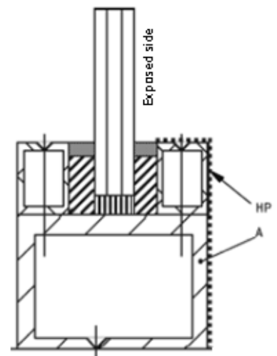
Schematic drawing 3
