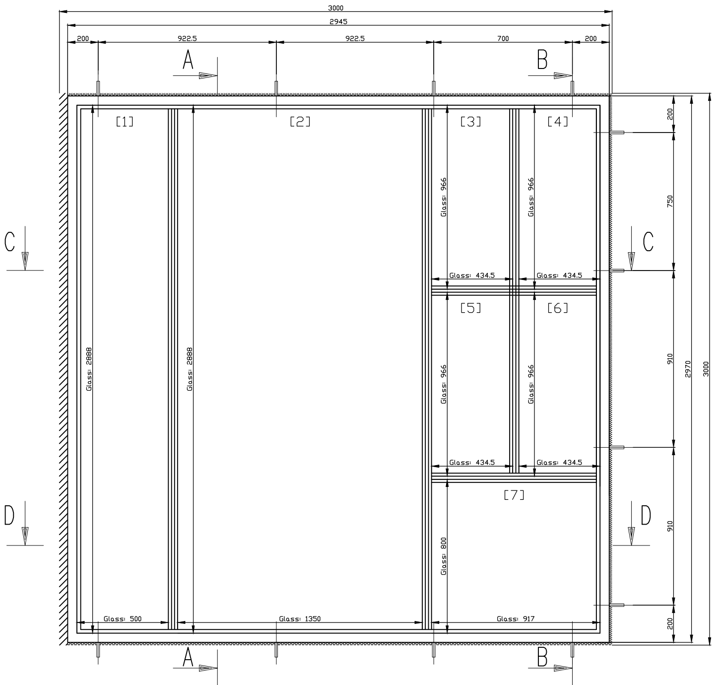
Front view (unexposed side) - dimensions
