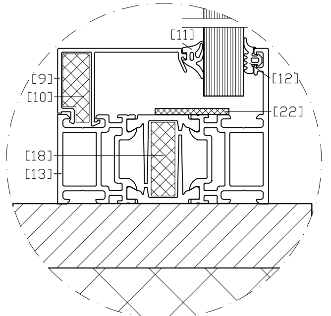
DETAIL D
