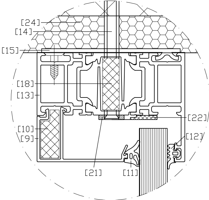
DETAIL C
